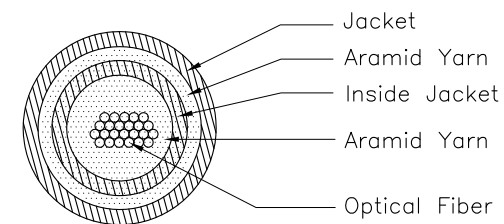
Cable Section (SCALE 5/1)
